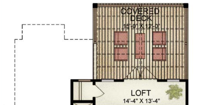
OPT'L COVERED DECK
